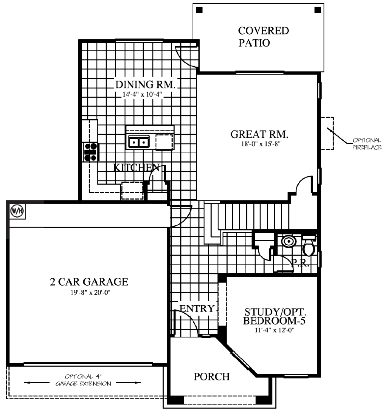
FIRST FLOOR
